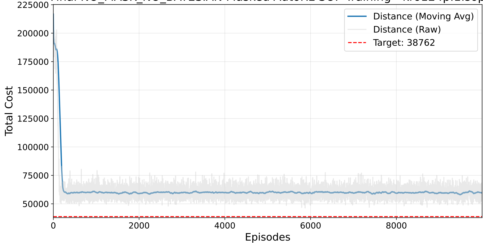
Final NO_MASK_NO_BAYESIAN Masked AutoRL-SOP Training - kro124p.1.sop
